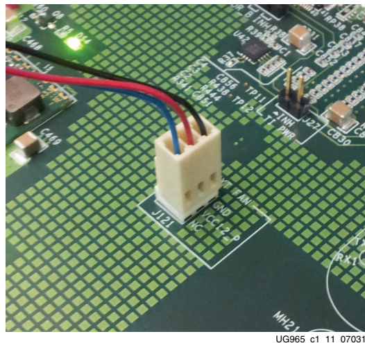
Figure 1-11: Heatsink Fan Power Connector J121
