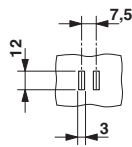
Dimensioned drawing
