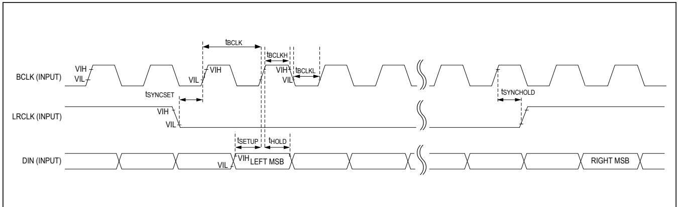
Figure 1. I²S Audio Interface Timing Diagram
