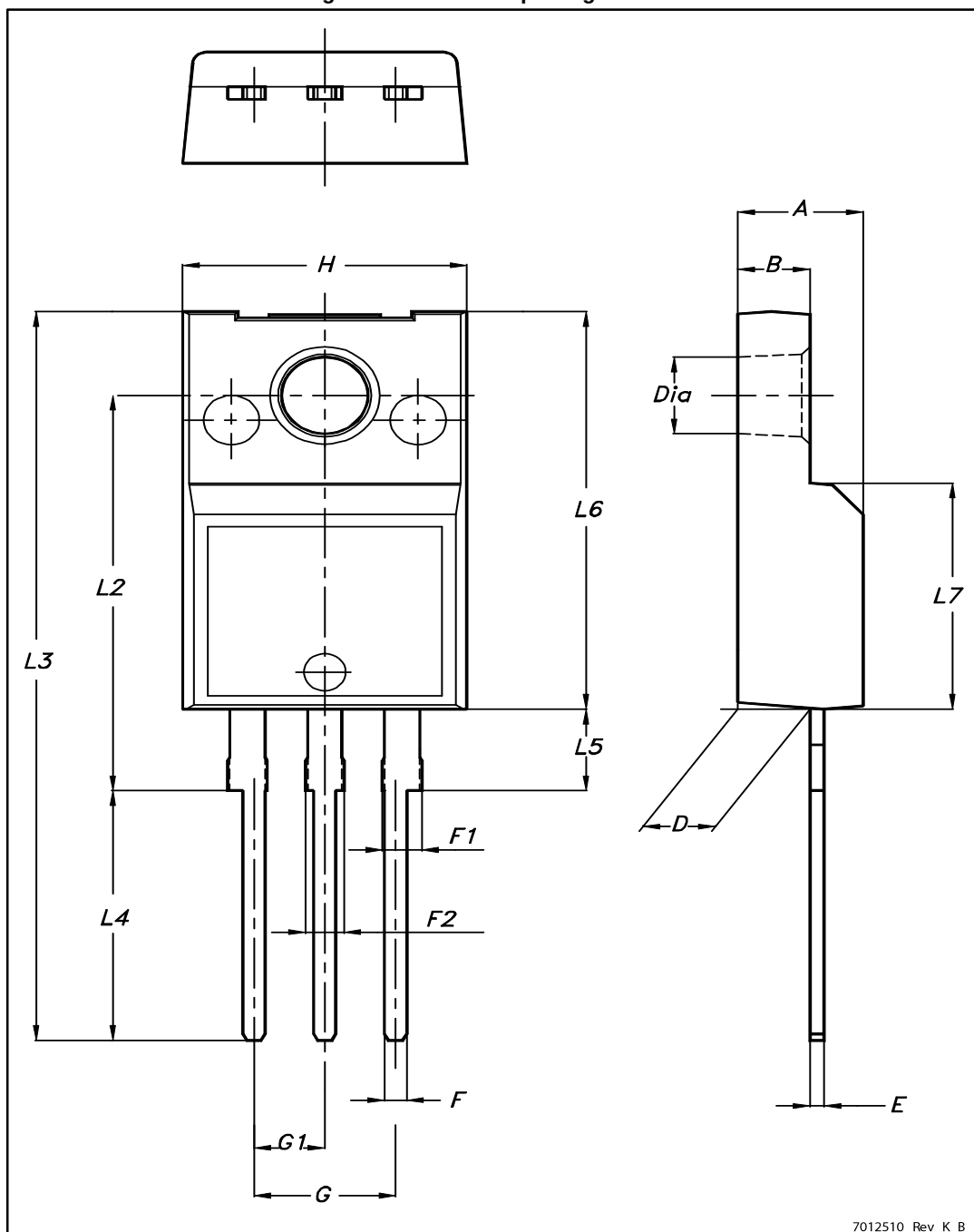
Figure 33: TO-220FP package outline
