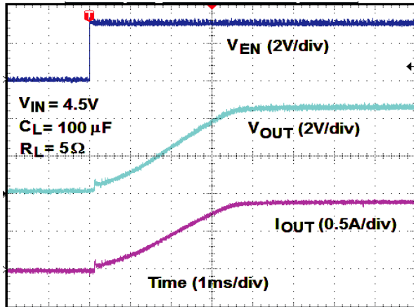
Figure 22 - Turn-On Time (V IN = 4.5 V, R L = 5 Ω, C L = 100 µF)
