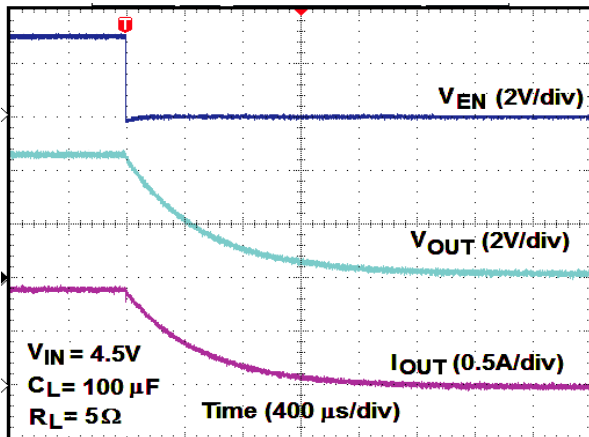
Figure 23 - Turn-Off Time (V IN = 4.5 V, R L = 5 Ω, C L = 100 µF)
