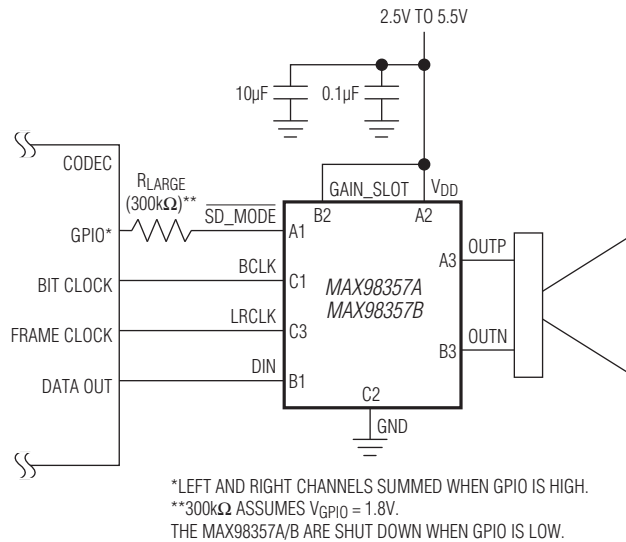
Figure 18. (Left/2 + Right/2) PCM Operation with 6dB Gain
