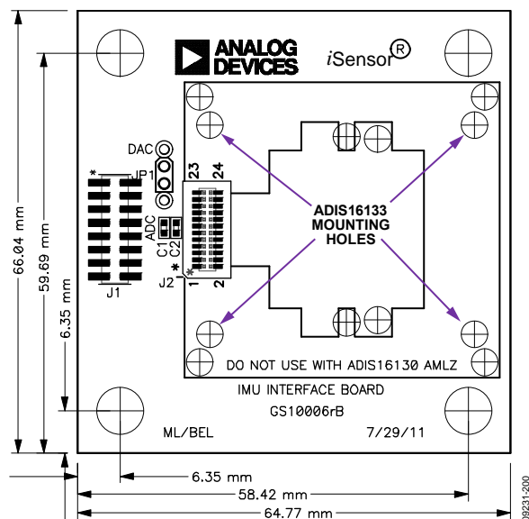
Figure 21. Physical Diagram for the Current ADIS16133/PCBZ
