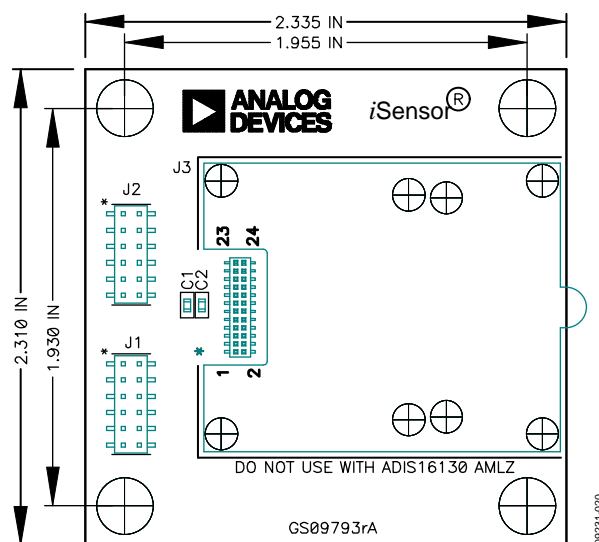
Figure 23. Physical Diagram for the ADIS16133/PCBZ
