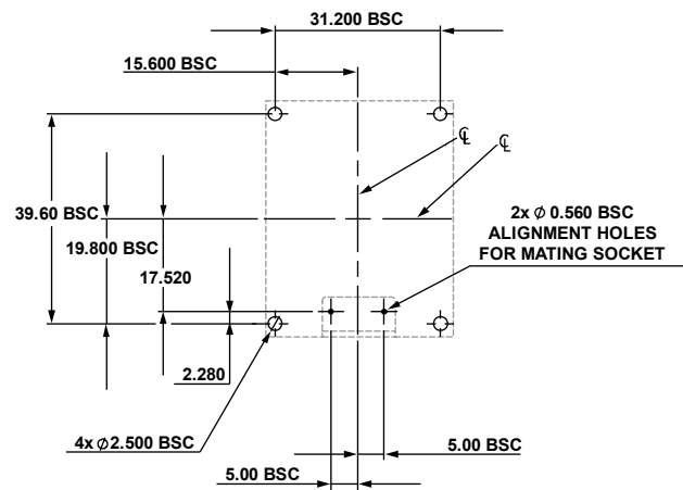
Figure 25. Suggested Mounting Hole Locations, Connector Down
