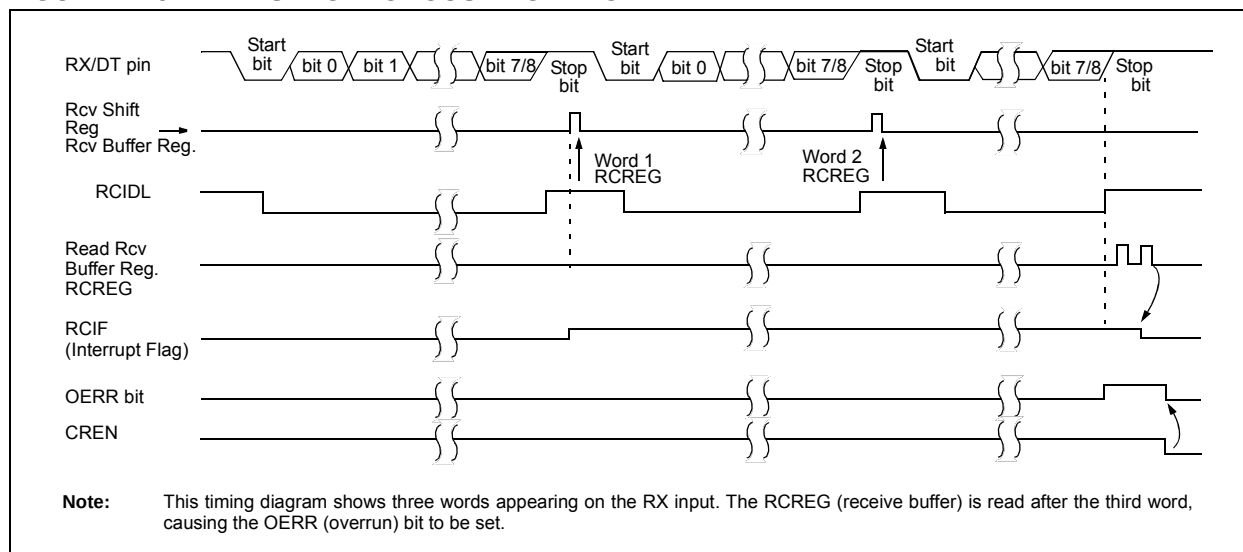
FIGURE 24-5: ASYNCHRONOUS RECEPTION
