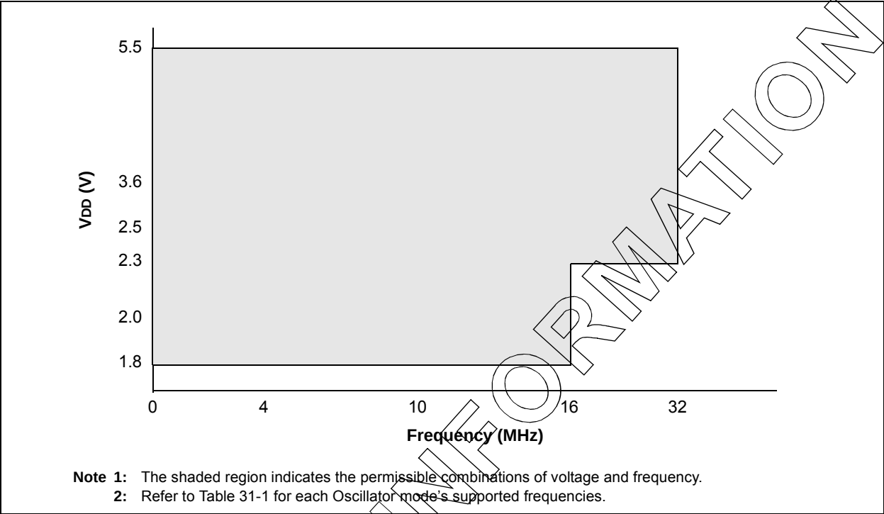
FIGURE 31-1: PIC16F/LF1938/39 VOLTAGE FREQUENCY GRAPH, -40°C ≤ Ta ≤ +125°C
