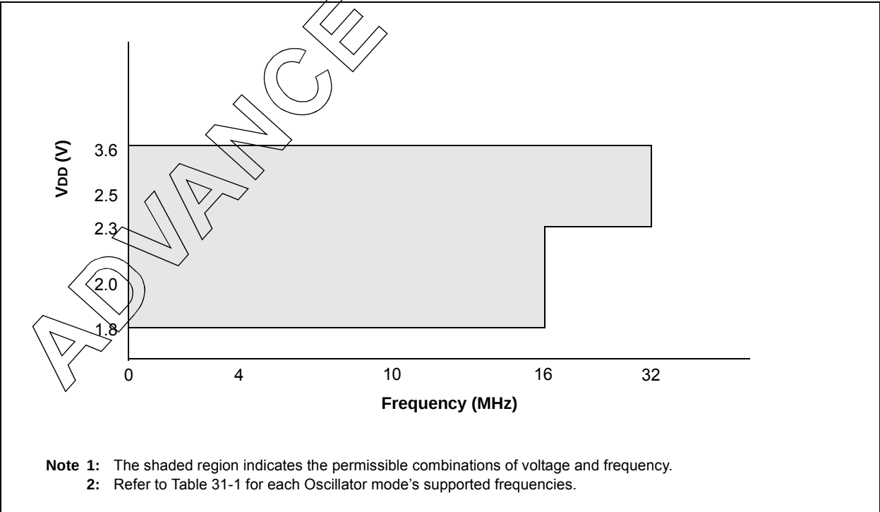
FIGURE 31-2: PIC16F/LF1938/39 VOLTAGE FREQUENCY GRAPH, -40°C ≤ Ta ≤ +125°C
