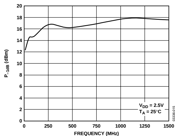
Figure 15. P -1dB vs. Frequency
