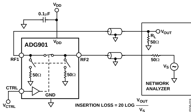
Figure 19. Insertion Loss
