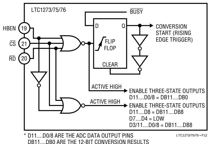
Figure 12. Internal Logic for Control Inputs \overline{CS} , \overline{RD} and HBEN
