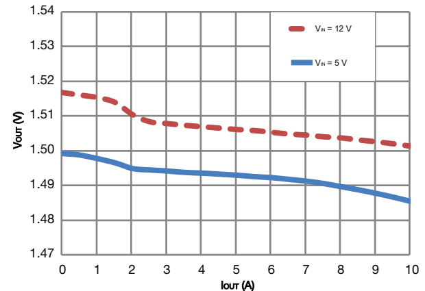
Figure 11 - Load Regulation - PSM (V DD = 3.3 V, V OUT = 1.5 V)
