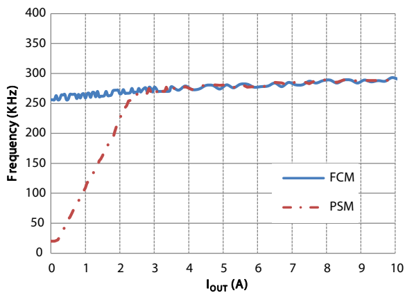
Figure 9 - Switching Frequency - PSM vs. FCM (V DD = 5 V, V OUT = 1.5 V, V IN = 12 V)
