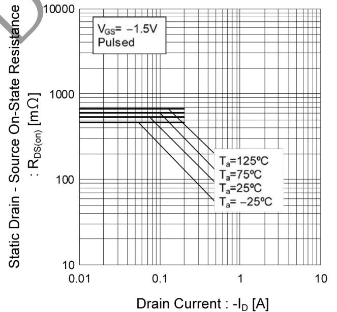
Fig.14 Static Drain - Source On - State Resistance vs. Drain Current (V)
