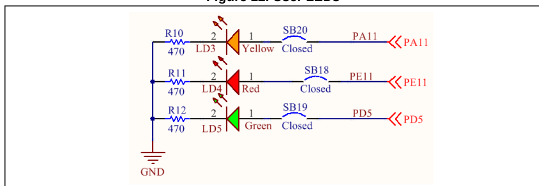
Figure 12. User LEDs
