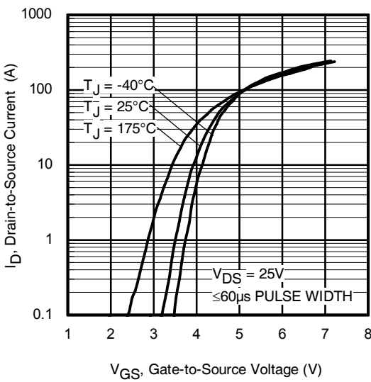
Fig 5. Transfer Characteristics
