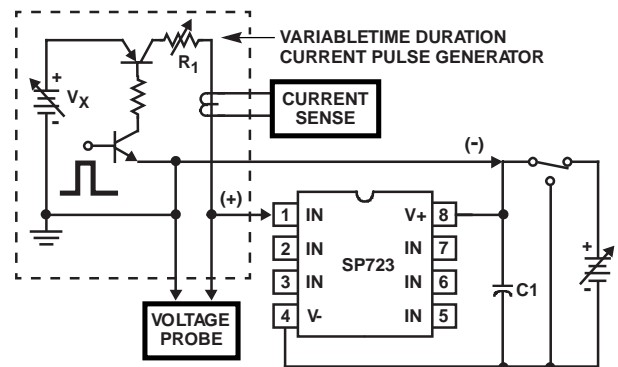
FIGURE 5. TYPICAL SP723 PEAK CURRENT TEST CIRCUIT WITH A VARIABLE PULSE WIDTH INPUT
