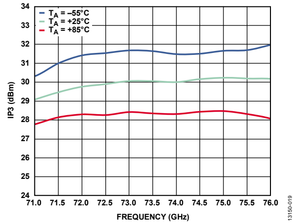
Figure 21. Output IP3 vs. Frequency at Various Temperatures, P_{IN} = -10 \text{ dBm/Tone} , V_{CTL1}/V_{CTL2} = -5 V
