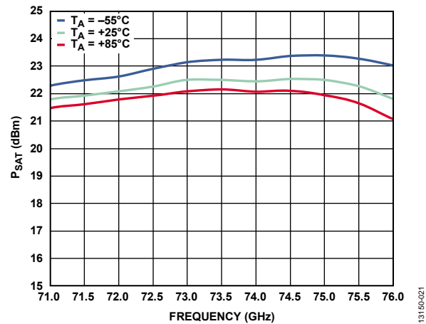
Figure 22. P_{SAT} vs. Frequency at Various Temperatures, V_{CTL1}/V_{CTL2} = -5 V
