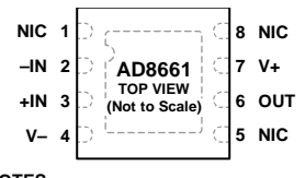
Figure 2. AD8661, 8-Lead LFCSP (CP-8-13)
