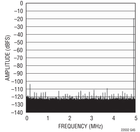
LTC2202: 128K Point FFT, f_{IN} = 5.1\text{MHz} , -20\text{dBFS} , PGA = 0, Internal Dither "Off"
