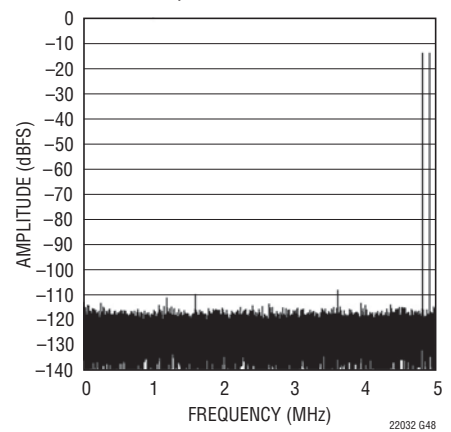
LTC2202: 32K Point 2-Tone FFT, f_{IN} = 5.1\text{MHz} and 15.2\text{MHz} , -15\text{dBFS} , PGA = 0
