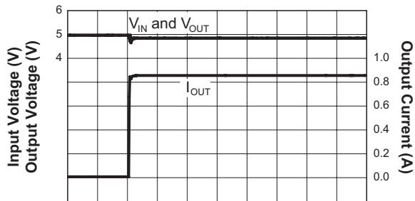
Soft Short Circuit with 5Ω Series Impedance ( V_{IN} = 5V )
