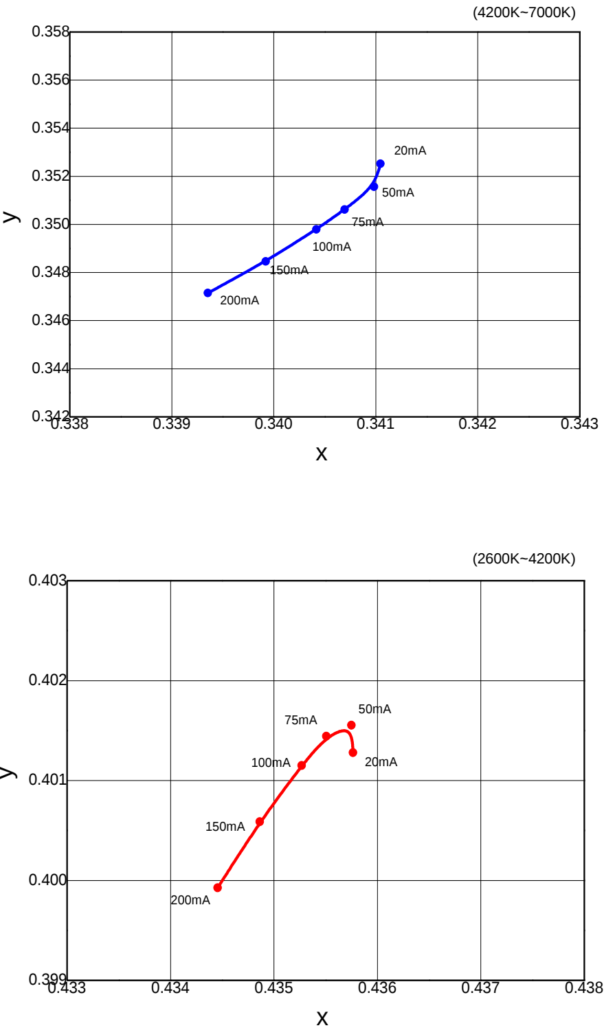
Fig 5. Forward Current vs. CIE X, Y Shift, T_j = 25^{\circ}\text{C}
