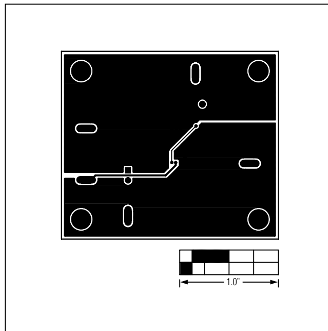
Figure 9. MAX17501G EV Kit PCB Layout—Solder Side
