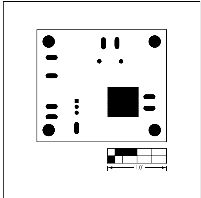
Figure 11. MAX17501G EV Kit PCB Layout—Bottom Solder Mask
