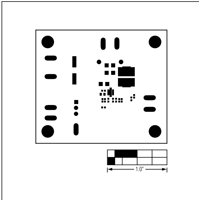
Figure 10. MAX17501G EV Kit PCB Layout—Top Solder Mask
