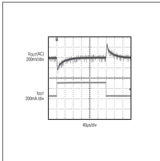
Figure 5. MAX17501G 250mA to 500mA Load Transient
