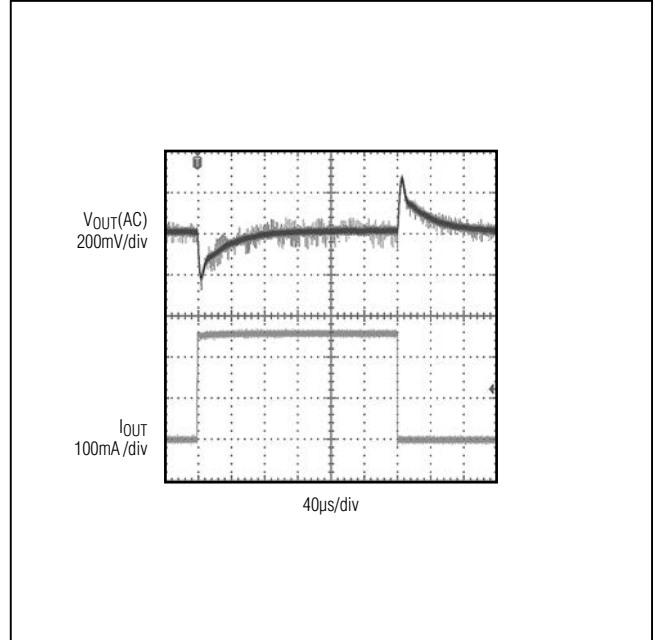
Figure 4. MAX17501G No Load to 250mA Load Transient
