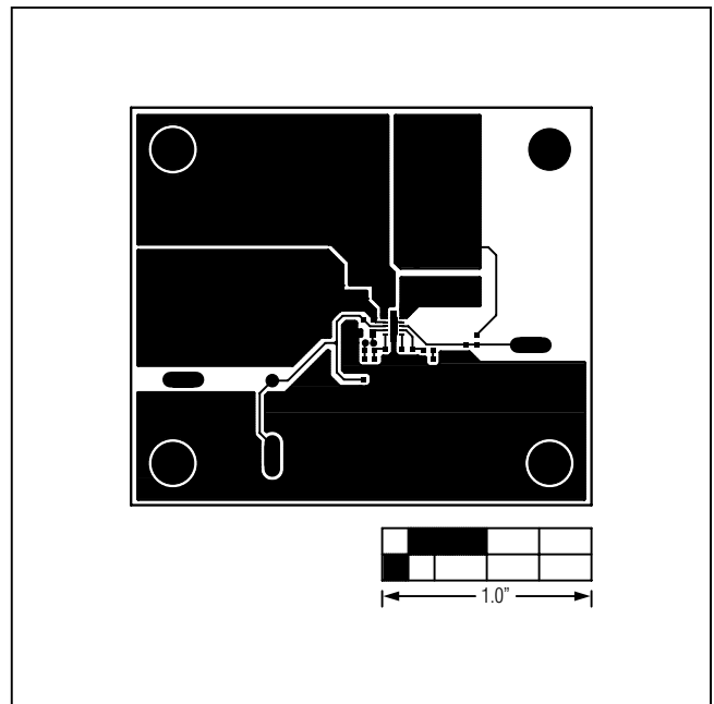
Figure 8. MAX17501G EV Kit PCB Layout—Component Side
