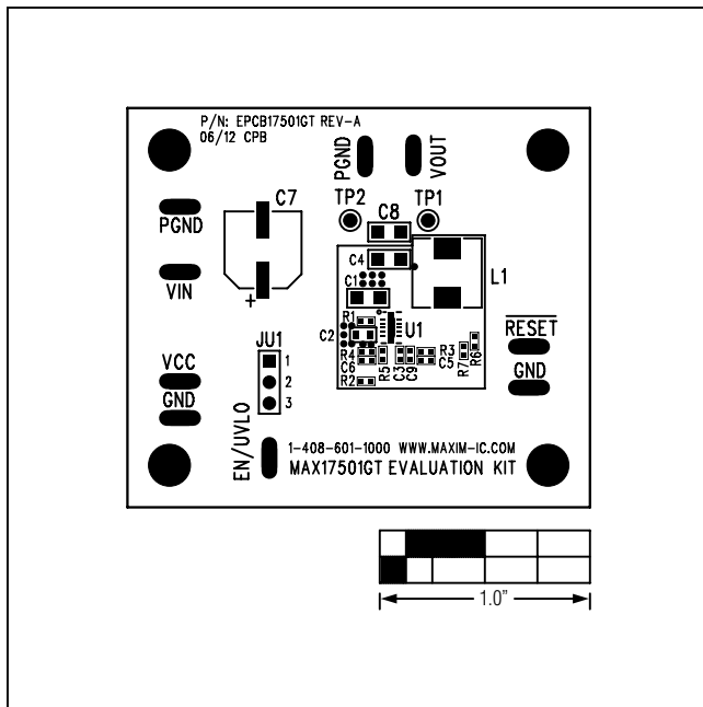
Figure 7. MAX17501G EV Kit Component Placement Guide—Component Side
