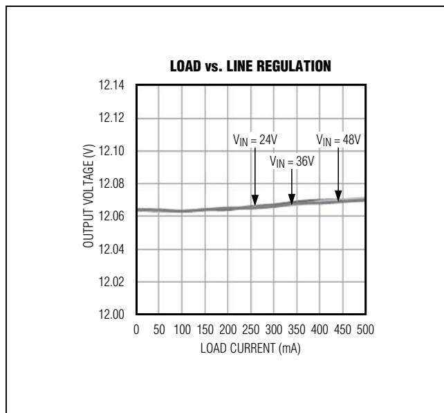
Figure 1. MAX17501G Load and Line Regulation
