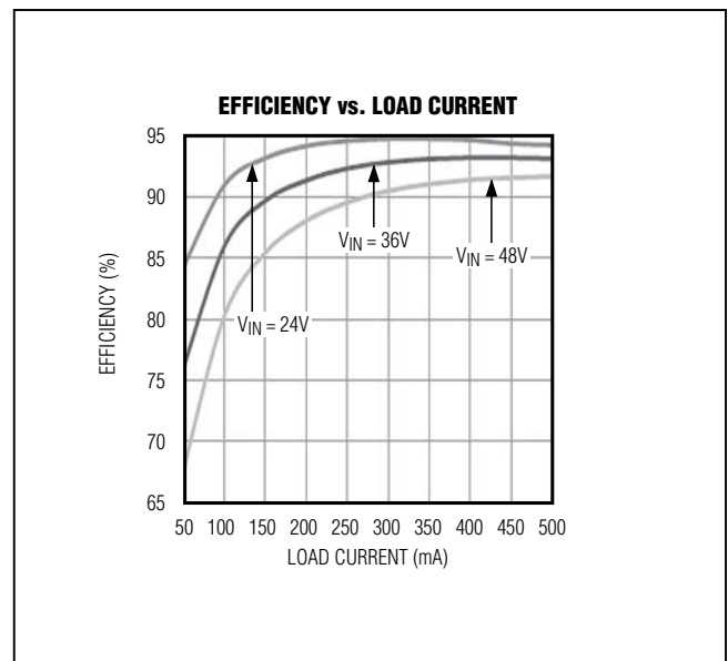
Figure 2. MAX17501G Efficiency
