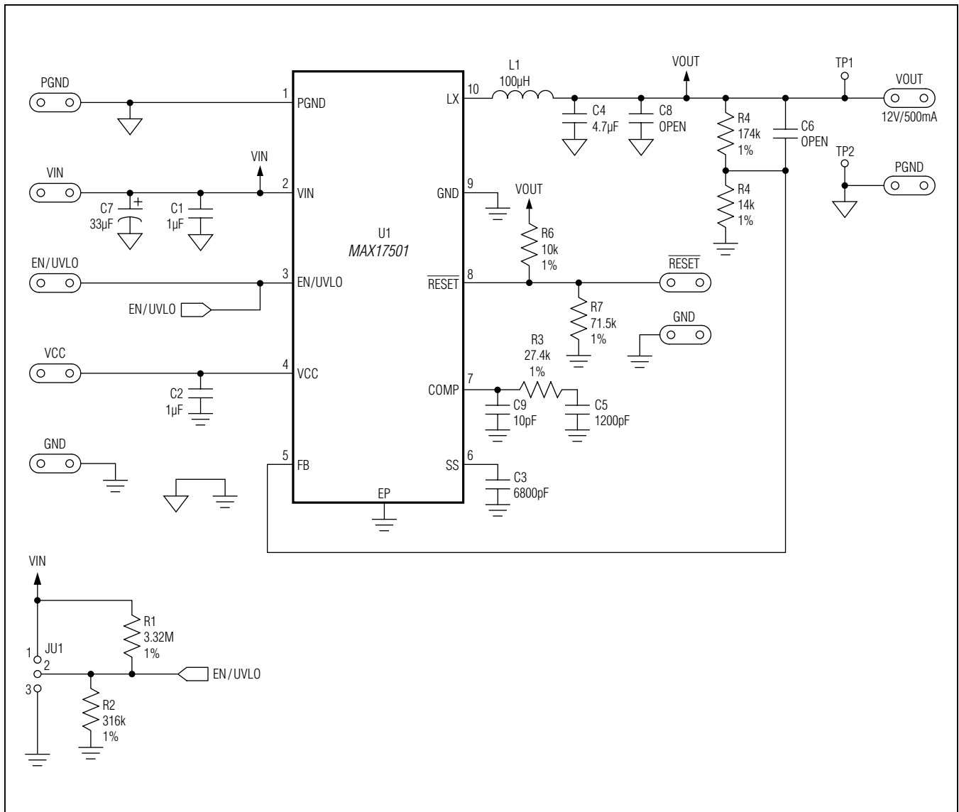
Figure 6. MAX17501G EV Kit Schematic
