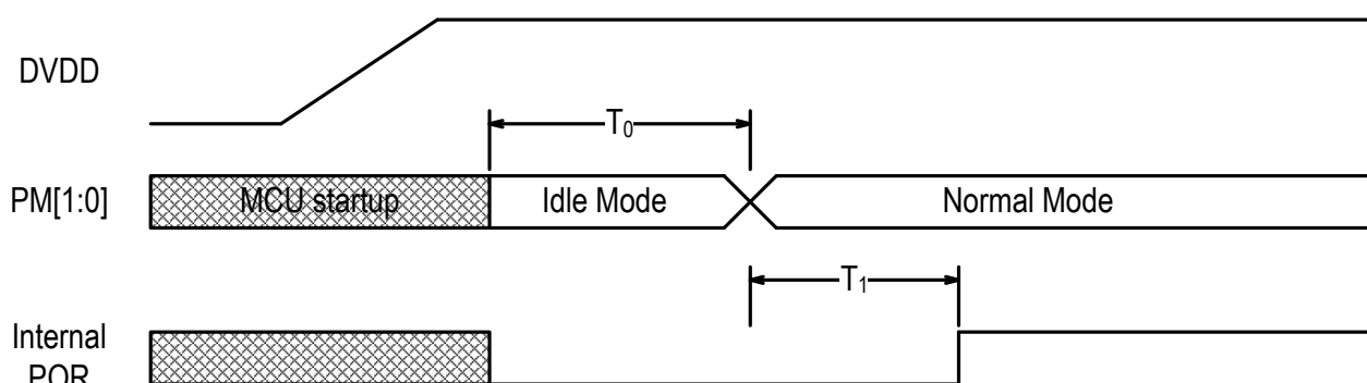
Figure-23 Power On Reset Timing (M90E32AS and MCU are Powered on Simultaneously)
