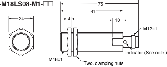
E2A-M18LS08-M1-□□
