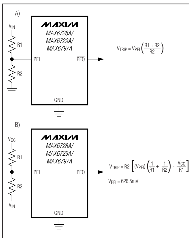
Figure 3. Using Power-Fail Input to Monitor an Additional Power-Supply a) V_{IN} is Positive b) V_{IN} is Negative
