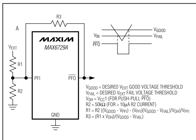
Figure 5. Adding Hysteresis to Power-Fail for Push-Pull \overline{\text{PFO}}
