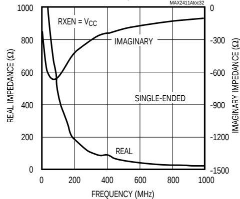
IF OR IF OUTPUT IMPEDANCE vs. FREQUENCY
