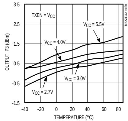
TRANSMIT MIXER OUTPUT IP3 vs. TEMPERATURE
