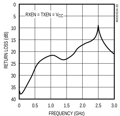
LO PORT RETURN LOSS vs. FREQUENCY
