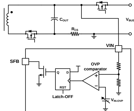
Figure 26 Output Over-Voltage Protection Block
