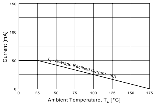
Figure 7. Average Rectified Current ( I_o ) versus Ambient Temperature ( T_A )
