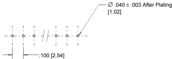
Recommended Hole Pattern
