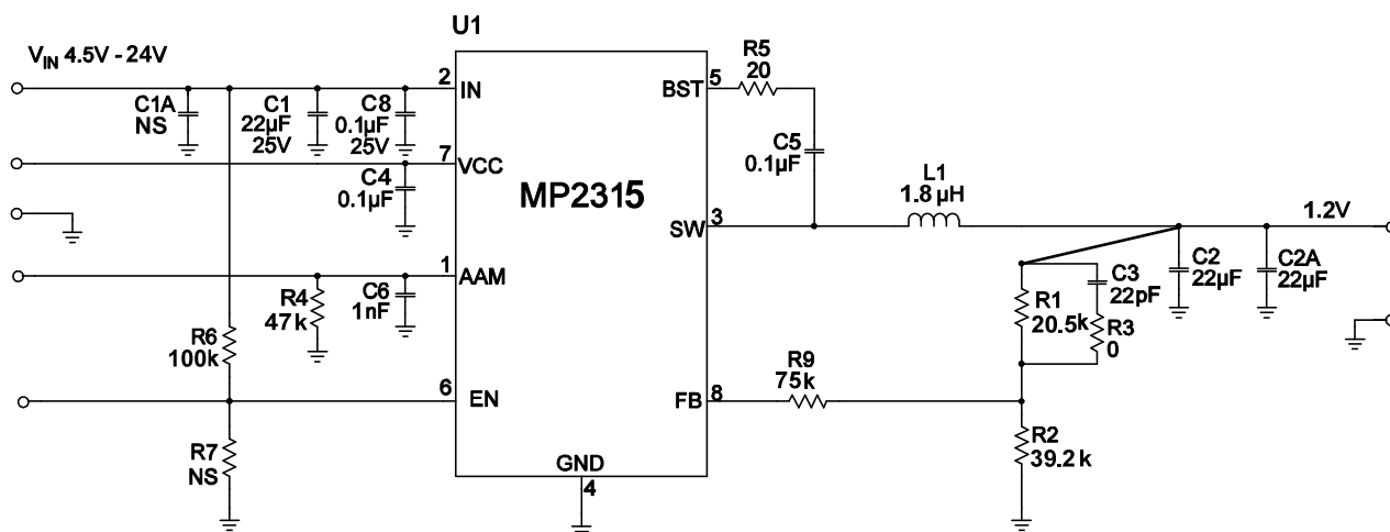
Figure 13: Vo=1.2V, Io=3A
