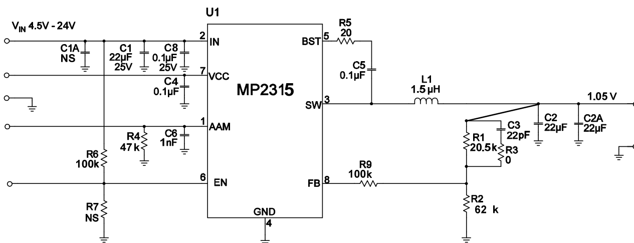
Figure 14: Vo=1.05V, Io=3A
