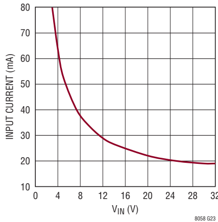
Input Current vs V_{IN} , V_{OUT1} Shorted
