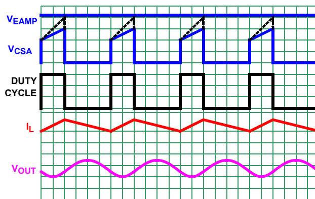
FIGURE 37. PWM OPERATION WAVEFORMS
