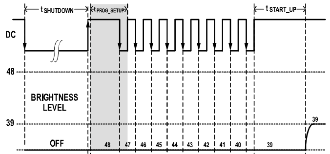
Figure 16. Presetting Timing
