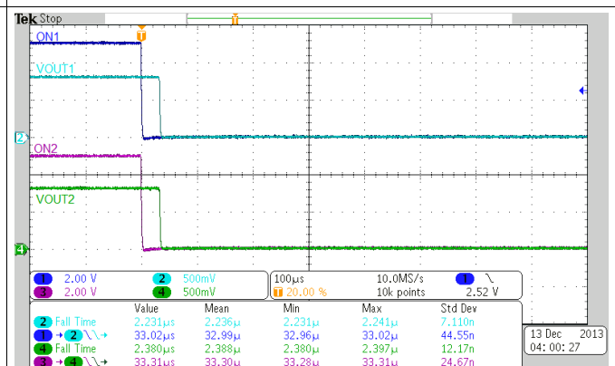
Figure 26. Turn-off Response Time (V_{IN} = 0.8\text{ V}, V_{BIAS} = 5\text{ V}, C_{IN} = 1\text{ }\mu\text{F}, C_L = 0.1\text{ }\mu\text{F}, R_L = 10\text{ }\Omega)
