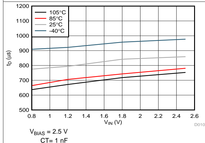
Figure 11. V_{IN} vs t_D
