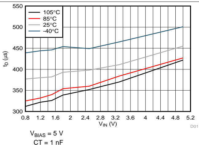
Figure 12. V_{IN} vs t_D
