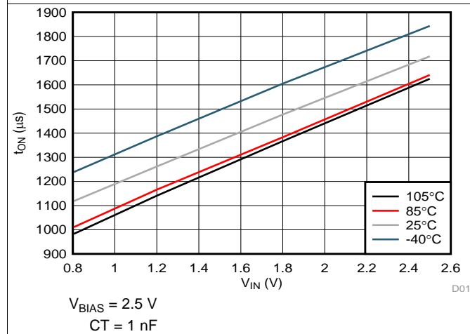
Figure 17. V_{IN} vs t_{ON}
