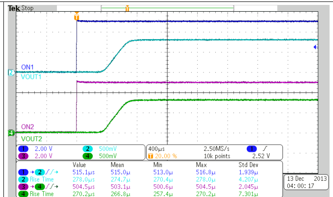
Figure 22. Turn-on Response Time (V_{IN} = 0.8\text{ V}, V_{BIAS} = 5\text{ V}, C_{IN} = 1\text{ }\mu\text{F}, C_L = 0.1\text{ }\mu\text{F}, R_L = 10\text{ }\Omega)
