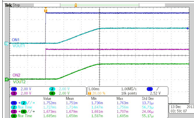
Figure 23. Turn-on Response Time (V_{IN} = 2.5\text{ V}, V_{BIAS} = 2.5\text{ V}, C_{IN} = 1\text{ }\mu\text{F}, C_L = 0.1\text{ }\mu\text{F}, R_L = 10\text{ }\Omega)
