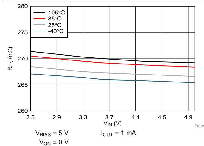
Figure 9. V_{IN} vs R_{PD} (TPS22968 Only) (Single Channel)
