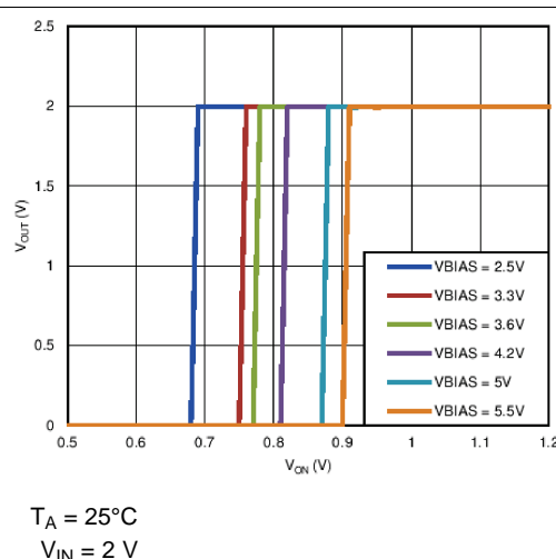
Figure 10. V_{ON} vs V_{OUT}
