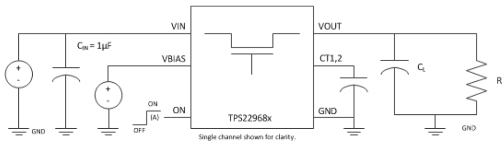
TEST CIRCUIT
