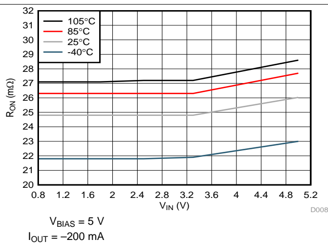
Figure 8. V_{IN} vs R_{ON}
