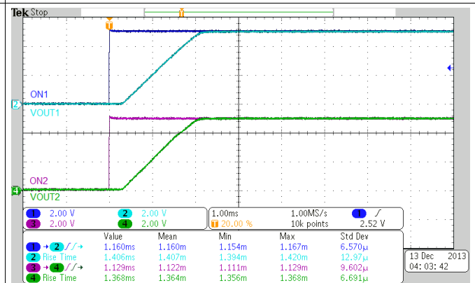
Figure 24. Turn-on Response Time (V_{IN} = 5\text{ V}, V_{BIAS} = 5\text{ V}, C_{IN} = 1\text{ }\mu\text{F}, C_L = 0.1\text{ }\mu\text{F}, R_L = 10\text{ }\Omega)
