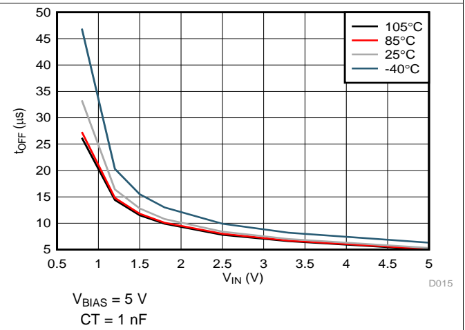
Figure 16. V_{IN} vs t_{OFF}
