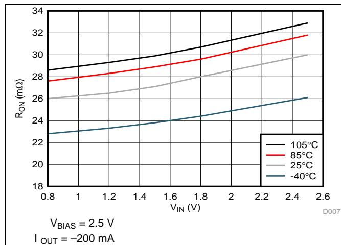
Figure 7. V_{IN} vs R_{ON}
