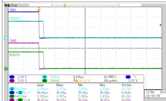
Figure 25. Turn-Off Response Time (V_{IN} = 0.8\text{ V}, V_{BIAS} = 2.5\text{ V}, C_{IN} = 1\text{ }\mu\text{F}, C_L = 0.1\text{ }\mu\text{F}, R_L = 10\text{ }\Omega)
