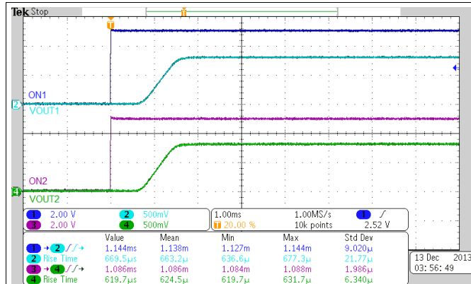
Figure 21. Turn-on Response Time (V_{IN} = 0.8\text{ V}, V_{BIAS} = 2.5\text{ V}, C_{IN} = 1\text{ }\mu\text{F}, C_L = 0.1\text{ }\mu\text{F}, R_L = 10\text{ }\Omega)
