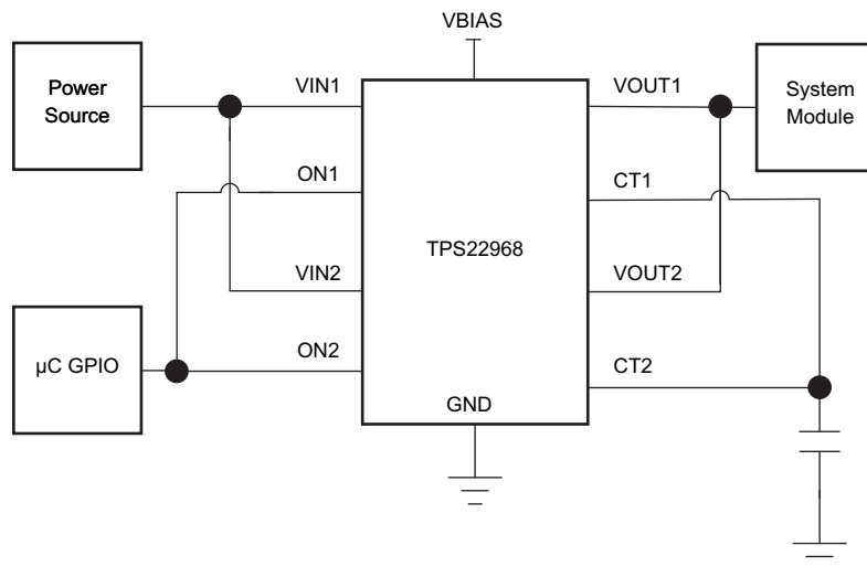
Figure 31. Parallel Configuration
