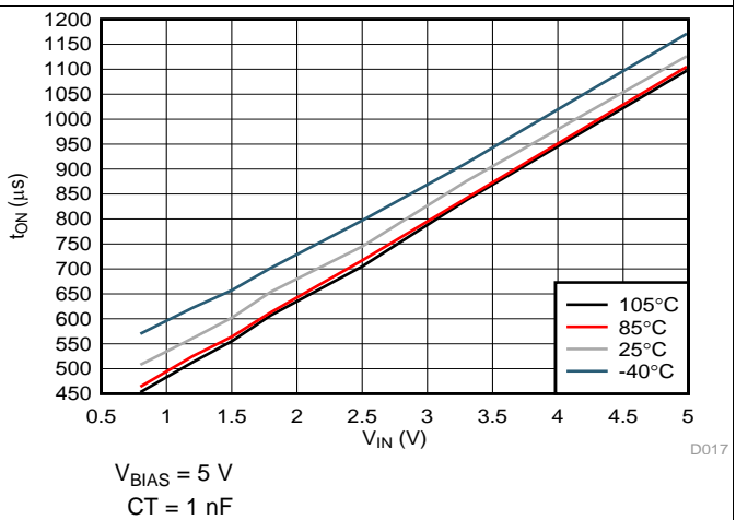
Figure 18. V_{IN} vs t_{ON}
