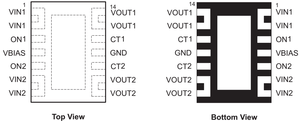
Pin Functions
