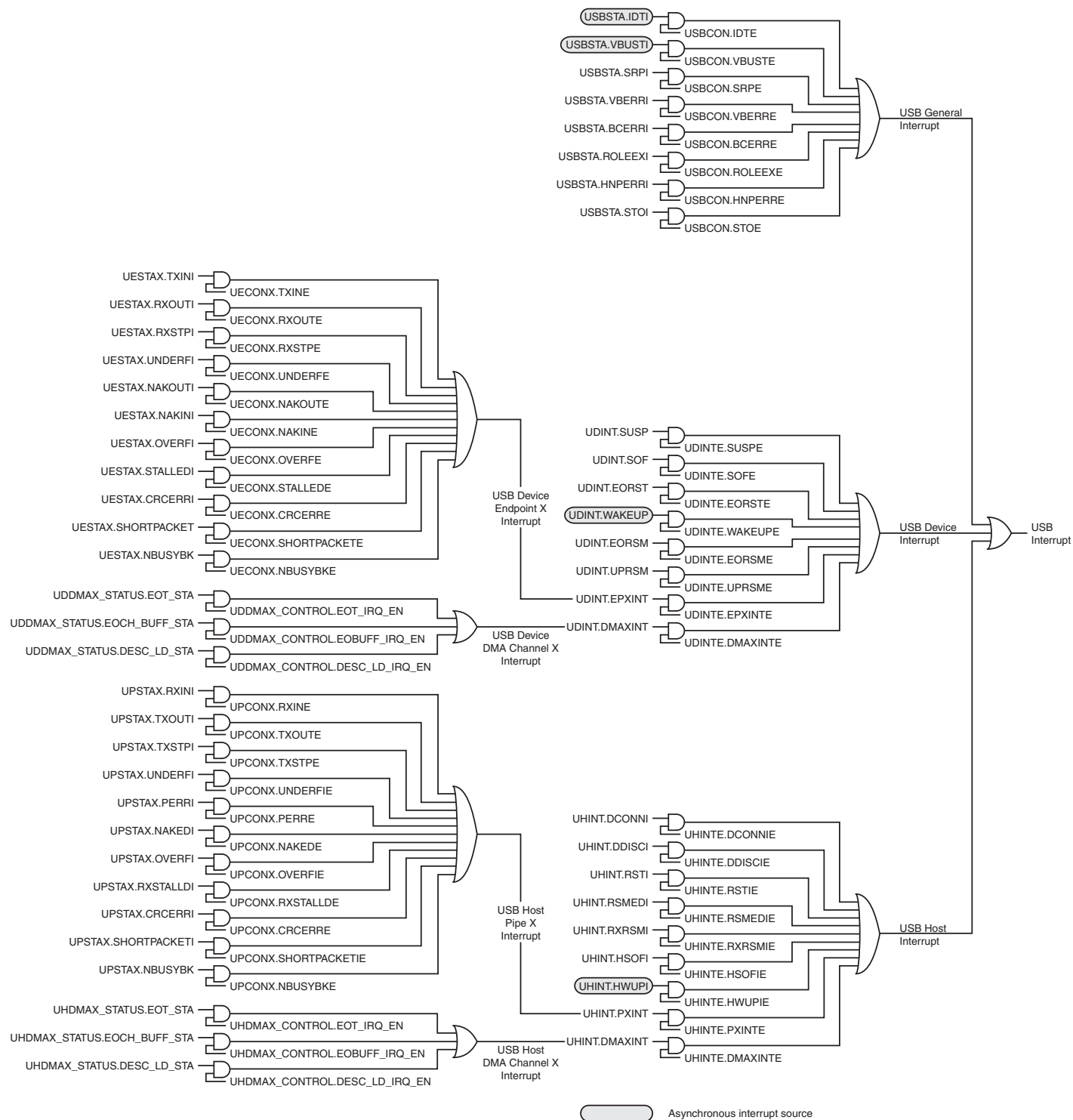
Figure 30-6. Interrupt System
