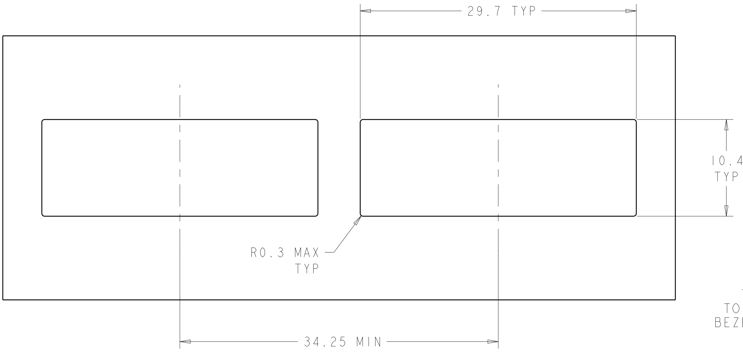
RECOMMENDED BEZEL CUT-OUT SCALE 4:1
