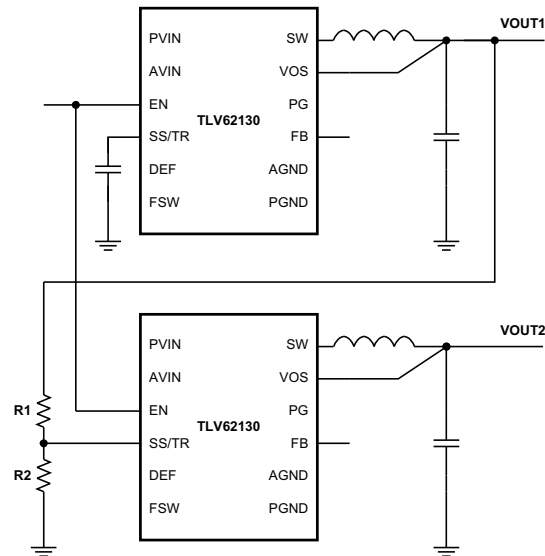
Figure 39. Sequence for Ratiometric and Simultaneous Startup
