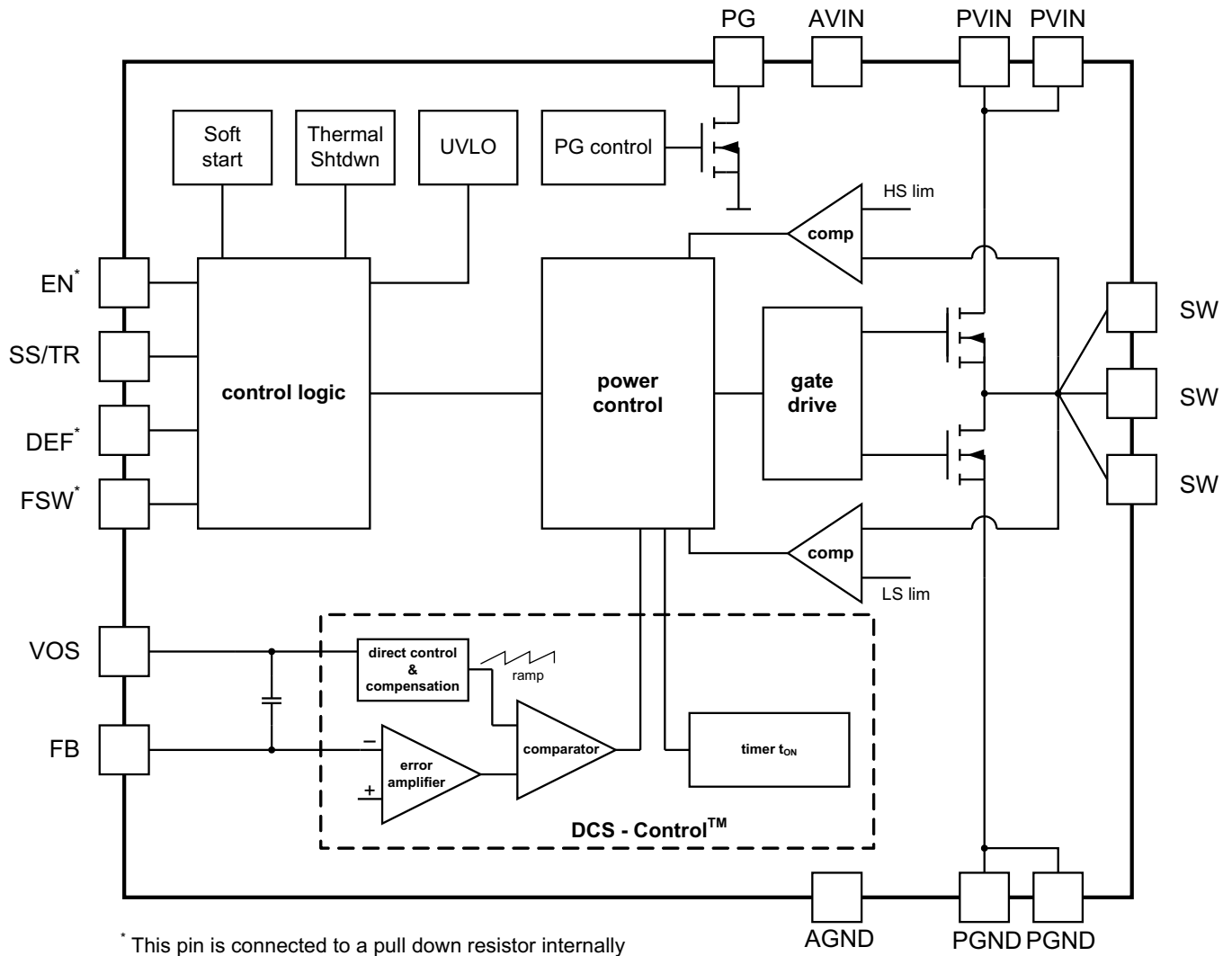
Figure 2. TLV62130
