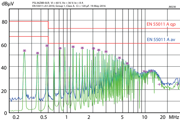
Fig. 12a PSL36Z8B: Conducted disturbances at the input according to EN 55011, group 1, class A, at V_i = 60\text{ V} , V_o = 36\text{ V} , I_o = 8\text{ A} ; external C_{ext} = 120\text{ }\mu\text{F} .
