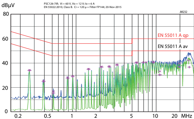
Fig. 11a PSC126-7iR: Conducted disturbances at the input as per EN 55011, at V_i = 60\text{ V} , V_o = 12\text{ V} , I_o = 6\text{ A} . External C_i = 120\ \mu\text{F} + Filter FP144.
