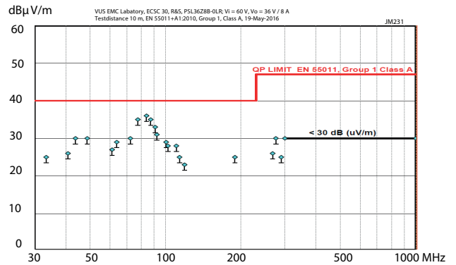
Fig. 12b PSL36Z8B: Radiated disturbances in 10 m distance, according to EN 55011, at V_i = 60\text{ V} , V_o = 36\text{ V} , I_o = 8\text{ A} ; external C_{ext} = 120\ \mu\text{F} .
