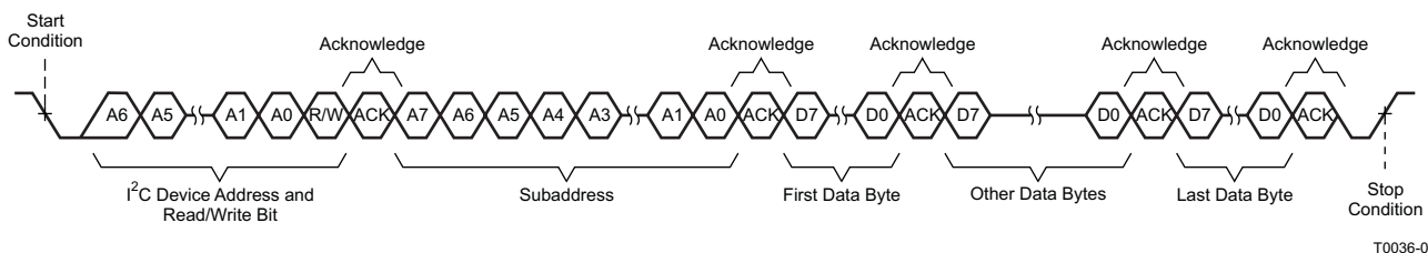
Figure 14. Sequential Write Transfer
