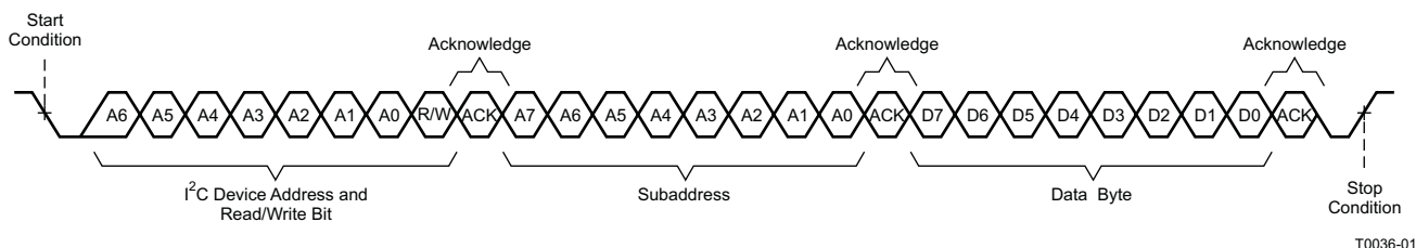
Figure 13. Random Write Transfer
