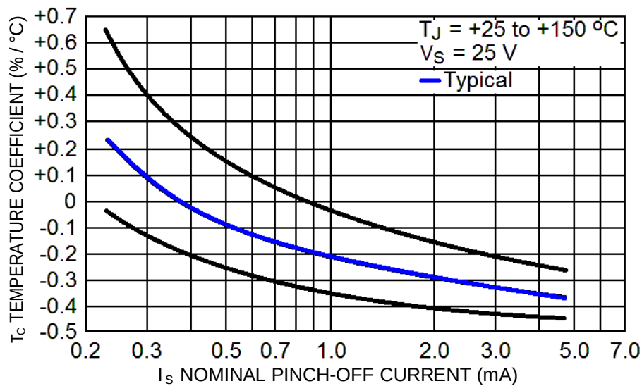
FIGURE 2 – TEMPERATURE COEFFICIENT
