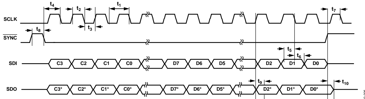
Figure 4. SPI Serial Interface Timing Diagram, CPOL = 0, CPHA = 1
