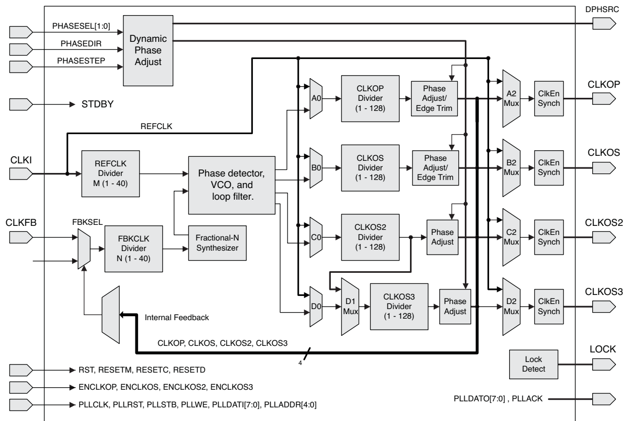
Figure 2-7. PLL Diagram
