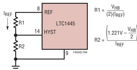
Figure 4. Programmable Hysteresis
