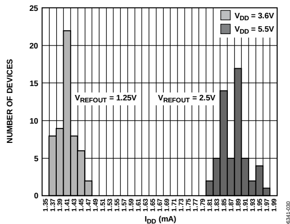
Figure 35. I_{DD} Histogram with Internal Reference
