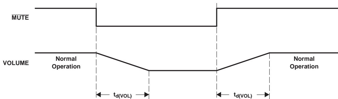
Figure 7-7. Mute Timing
