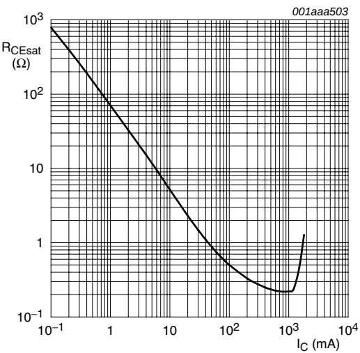
Fig 15. Equivalent on-resistance as a function of collector current; typical values
